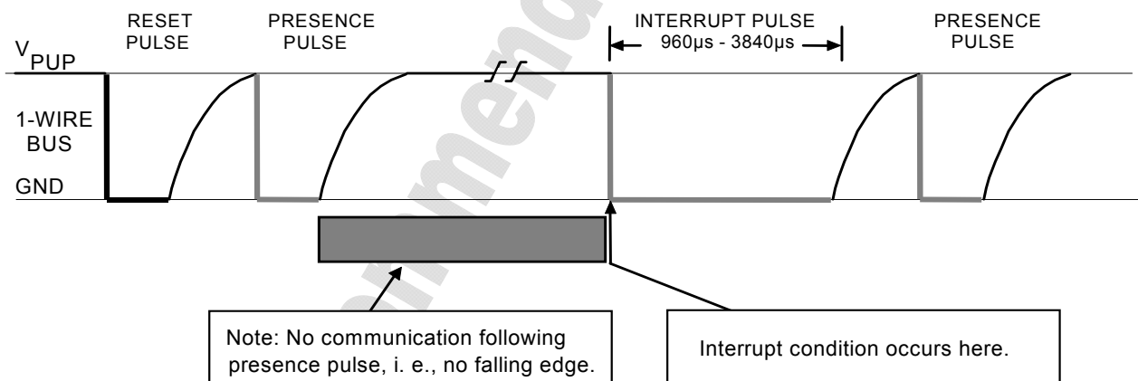
Figure 12. TYPE 1 INTERRUPT
