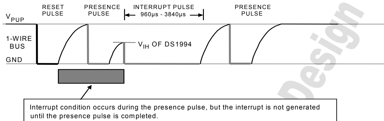
Figure 14. TYPE 2 INTERRUPT
