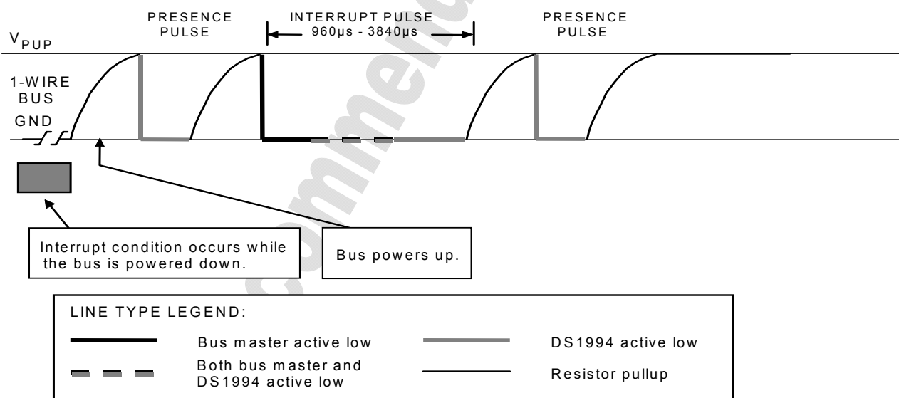
Figure 15. TYPE 2 INTERRUPT (SPECIAL CASE)
