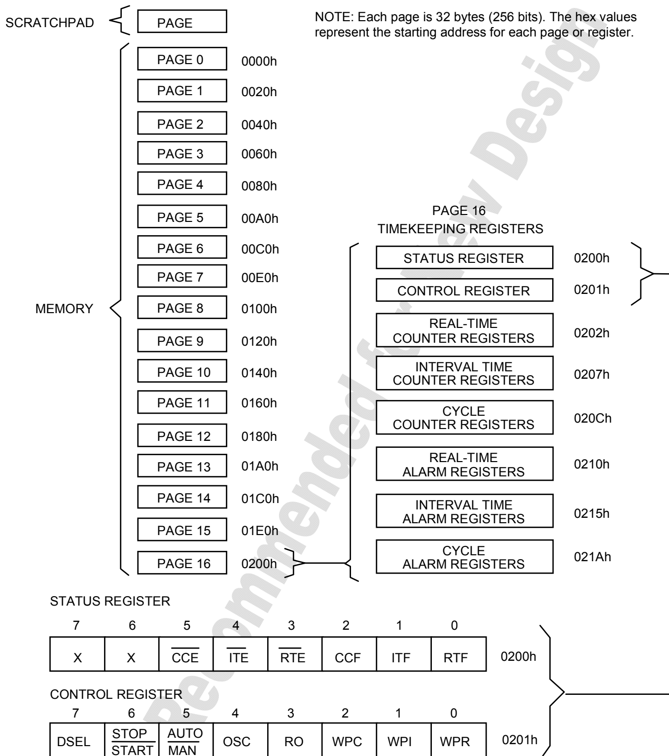
Figure 4. DS1994 MEMORY MAP
